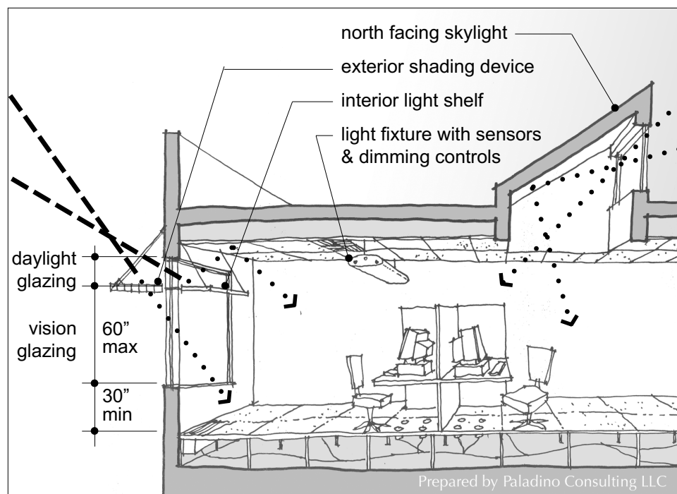
Figure 1: An Illustration of Various Daylighting Strategies
